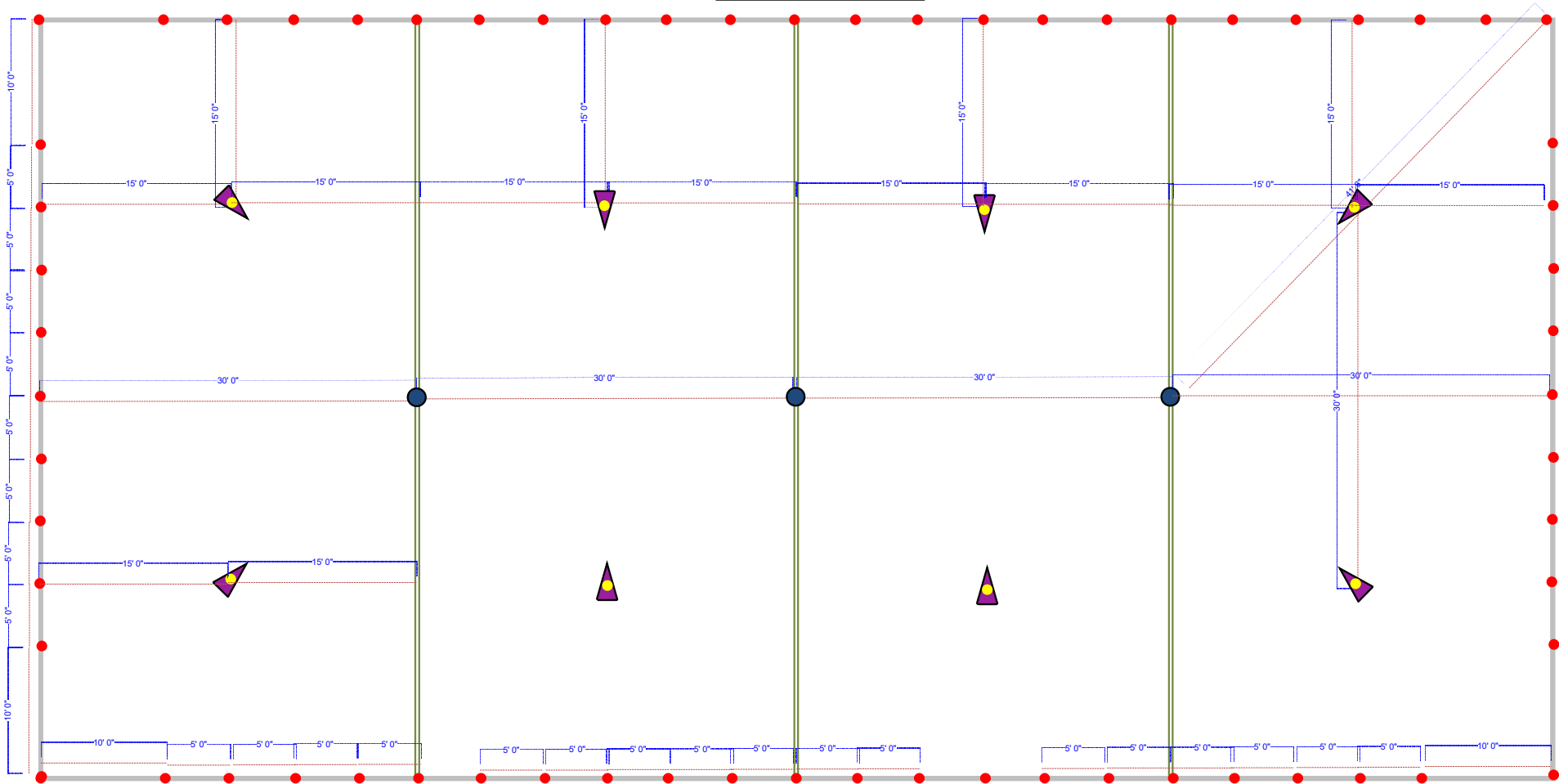
60' x 120' Pole Tent - Pole Placements
